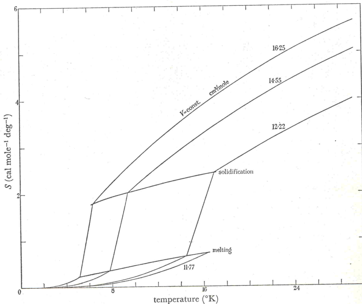
FIGURE 9. The entropy of 4 He. The numbered lines are lines of constant volume.
